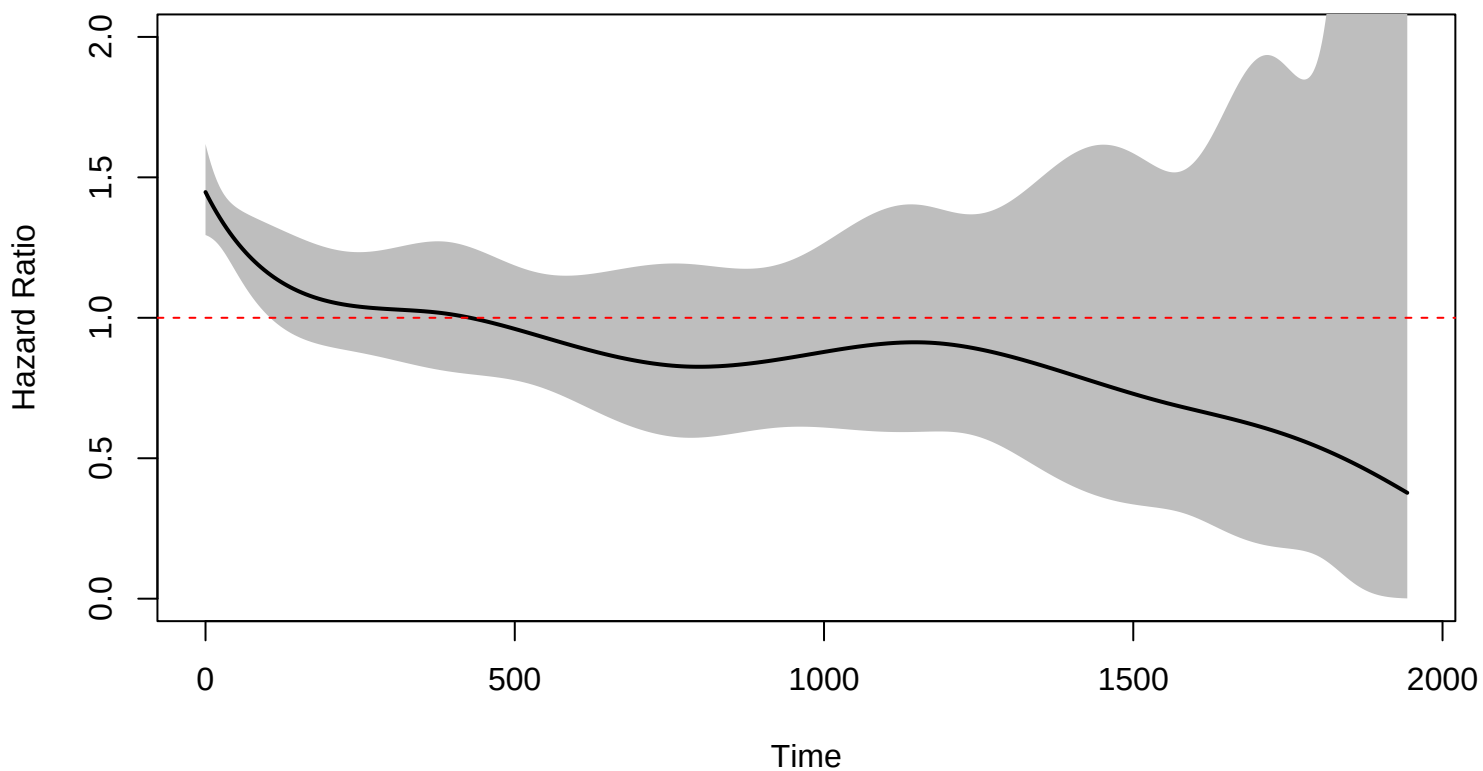
Model 8: Variable Hazard Ratio
